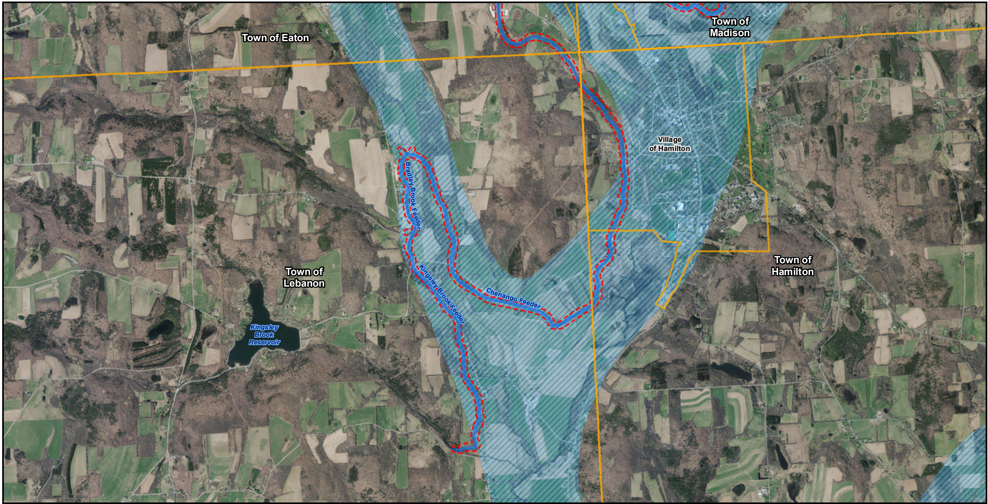
Figure 56F: Aquifers
